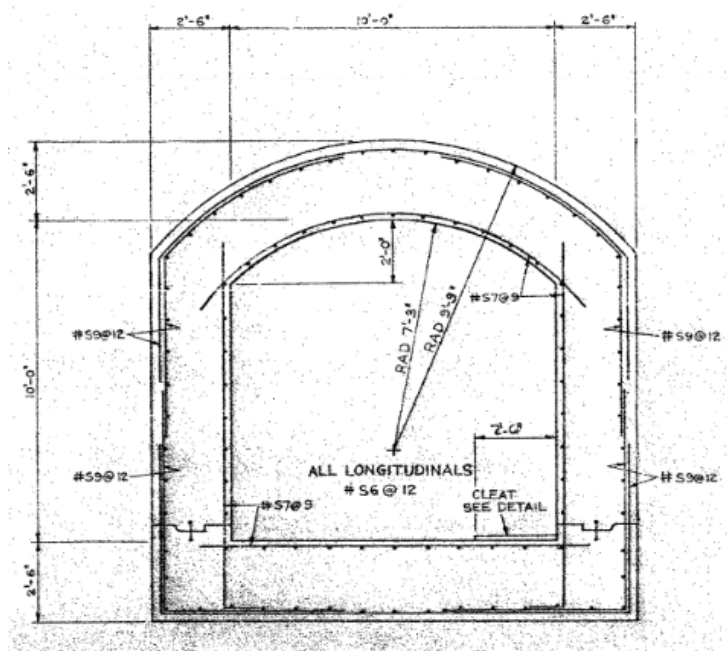
Section view of the tunnel
