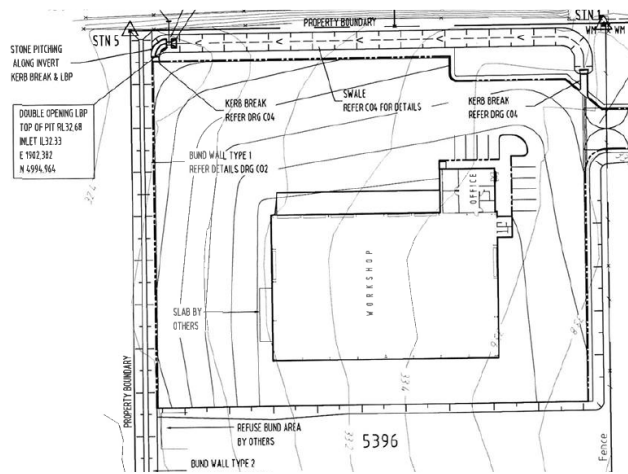
Site plan layout
