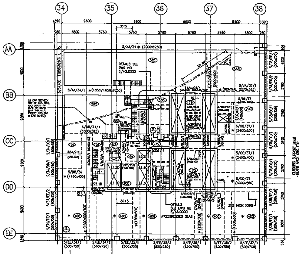
Layout of the transfer floor
