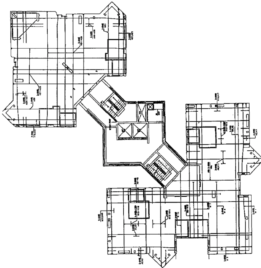
Plan layout: typical floor of the tower block: post-tensioning layout
